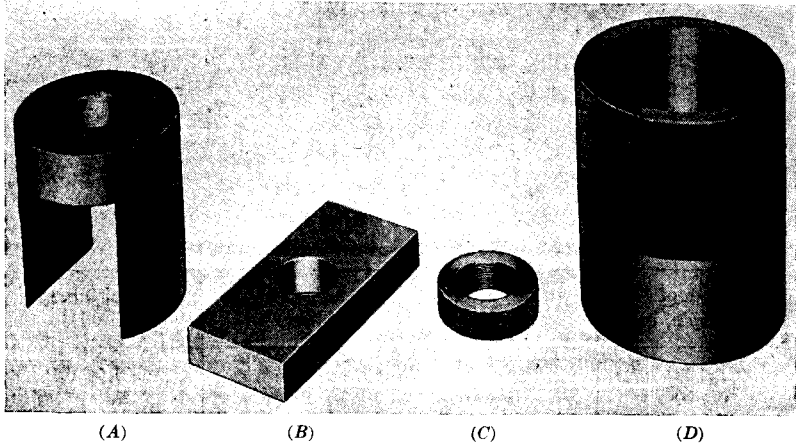
FIG. 17-7.—Stripping tools.
